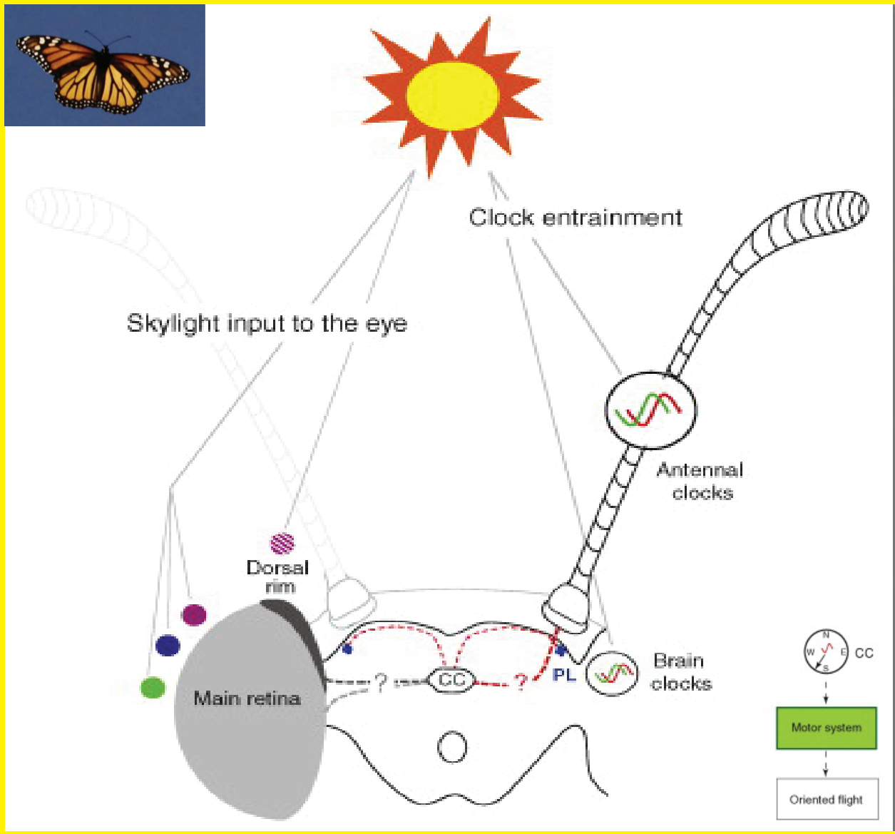
Model of the components and potential circuitry involved in the timecompensated sun compass mechanism. (From Trends in Neurosciences 2010 33:399-406; Abstract No. 61 in this issue. Free).
