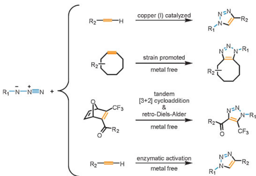
■ Scheme 1. General scheme of “click” chemistry cycloaddition reactions.
