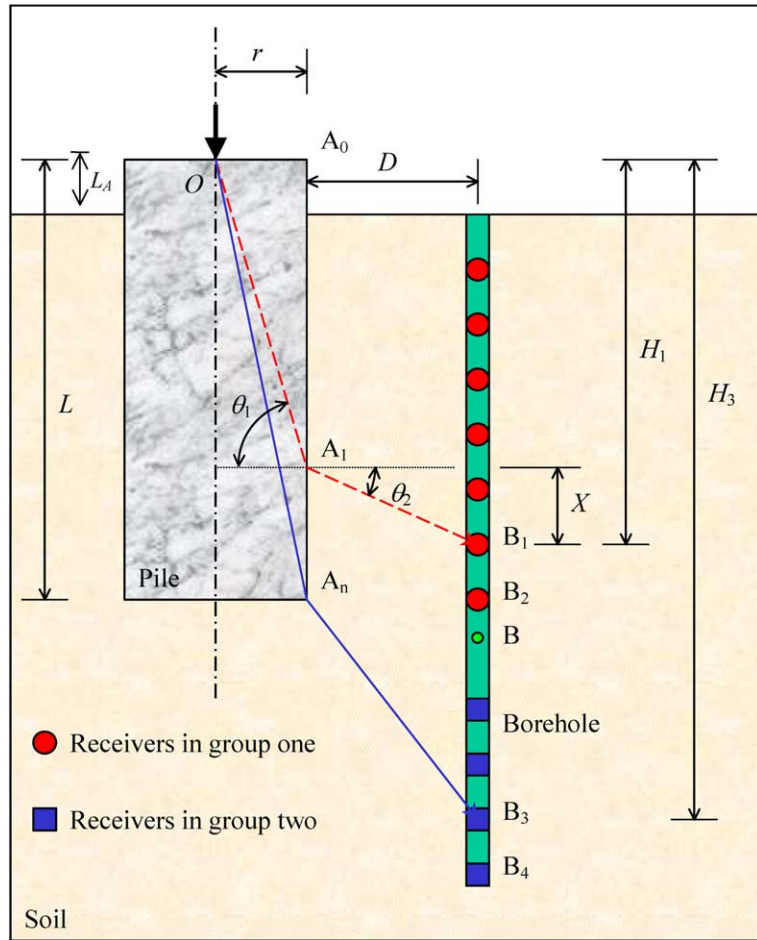
Fig. 6. Traveling paths of stress waves in a Parallel Seismic test.
