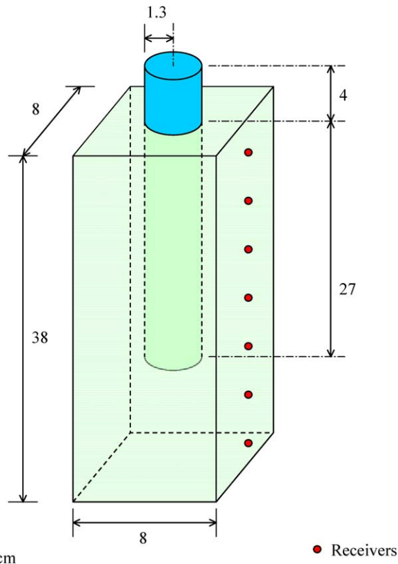
Fig. 8. Geometric configuration of the experimental model for a PS test.
