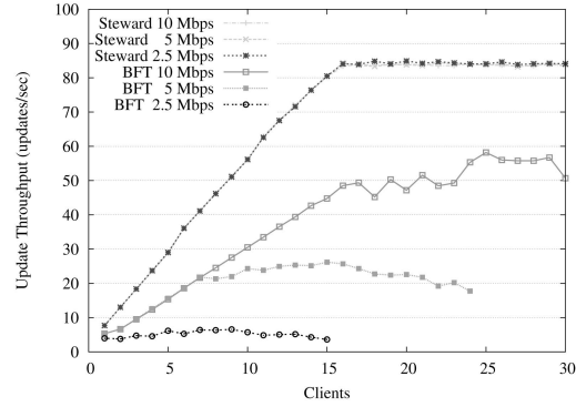
Fig. 4. Write update throughput.
