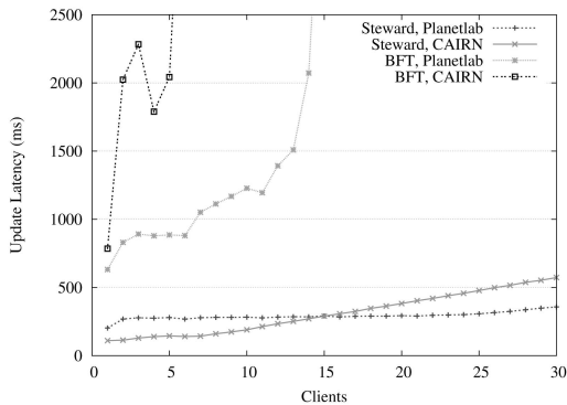
Fig. 9. WAN emulation—write update latency.
